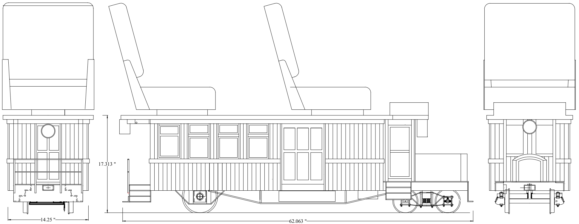
Railbus
